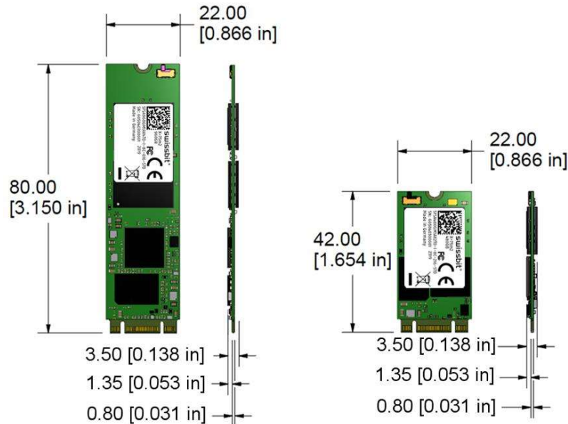
Figure 3: X-75m2 SATA SSD Dimensions in mm [in]
