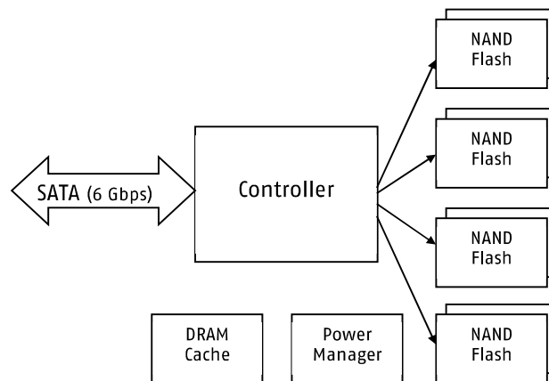
Figure 1: X-75m2 SATA Functional Block Diagram
