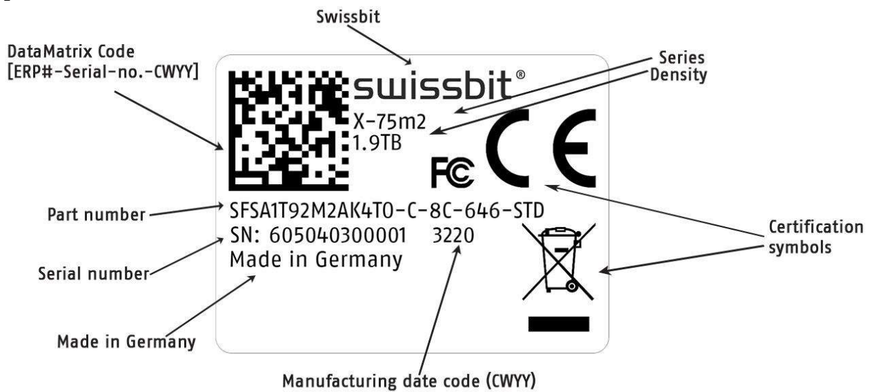
Figure 6: X-75m2 label details
