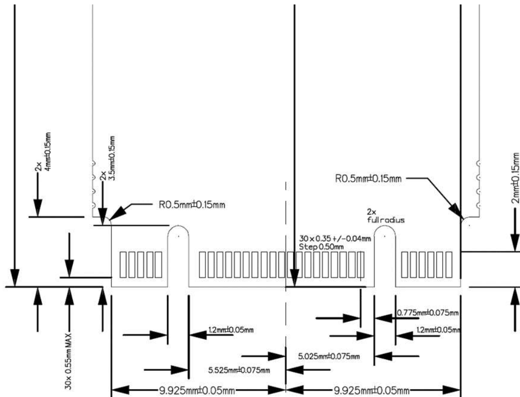
Figure 4: M.2 Connector Dimensions in mm
