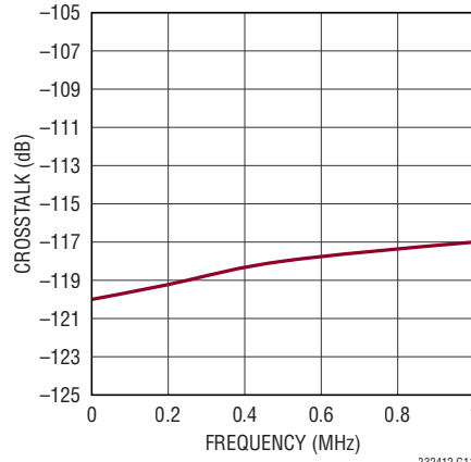
Crosstalk vs Input Frequency
