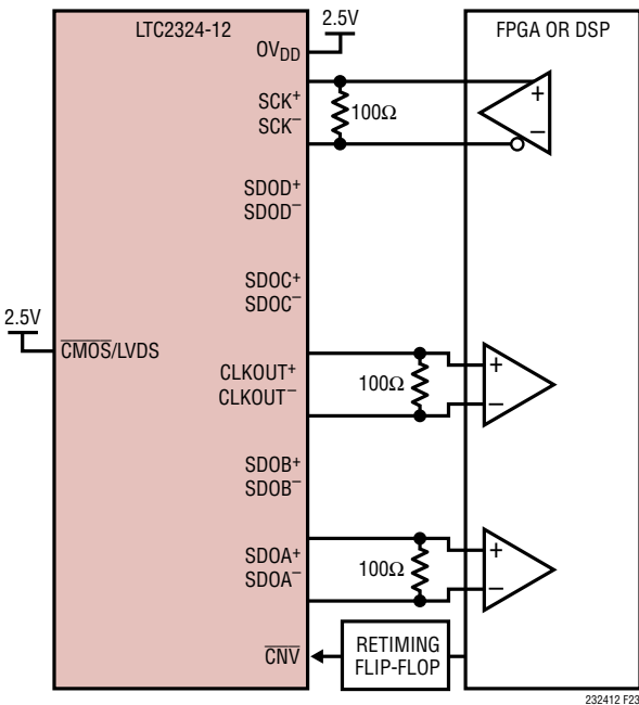
Figure 23. LTC2324-12 Using the LVDS Interface with One Lane
