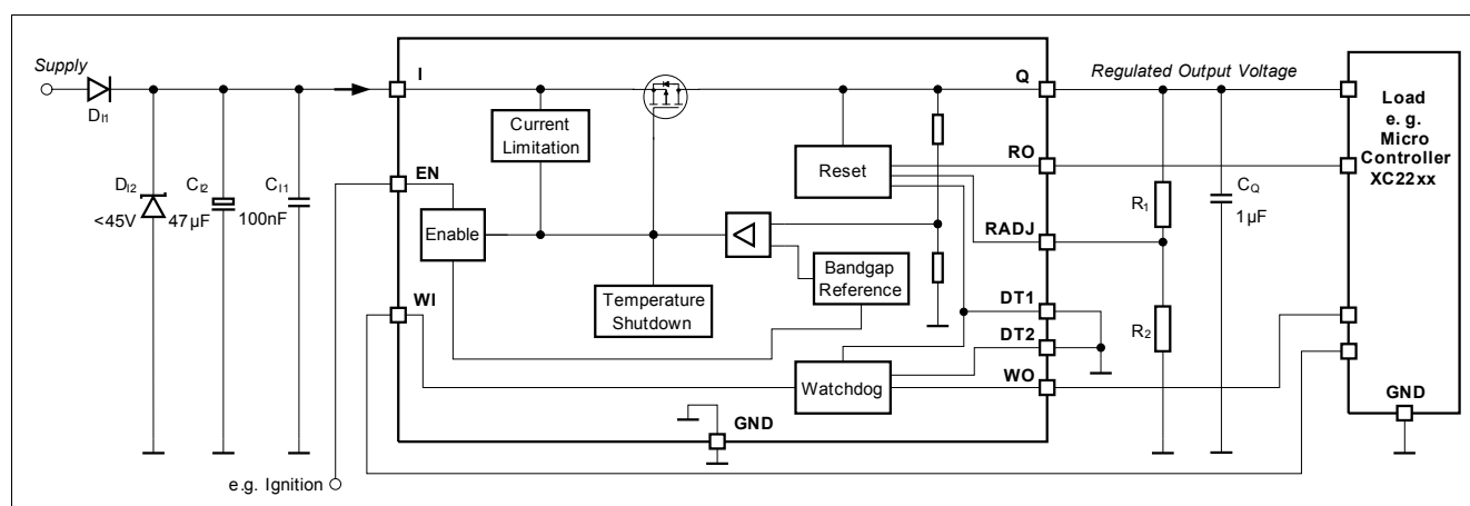
Figure 12 Application Diagram
