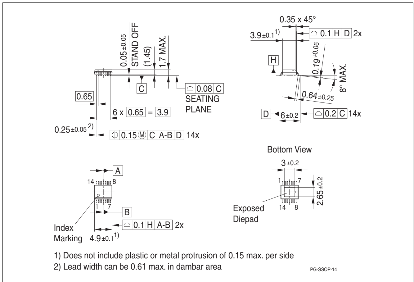
Figure 13 PG-SSOP-14
