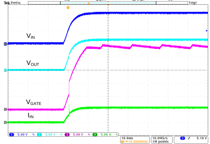
Start-up with 6A Load
