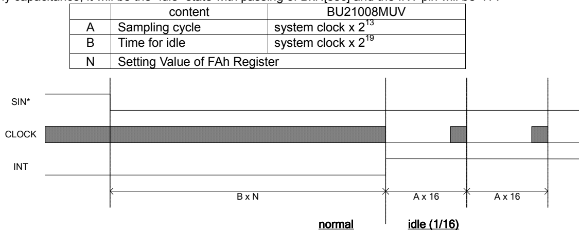
INT pin condition 1 (normal → idle)
