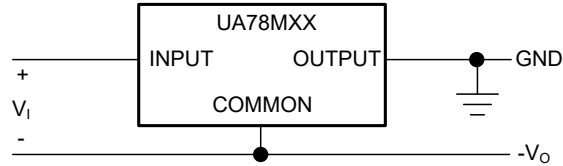
Figure 7-10. Positive Regulator in Negative Configuration
