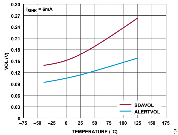
Figure 51. SDA/ALERT VOL
