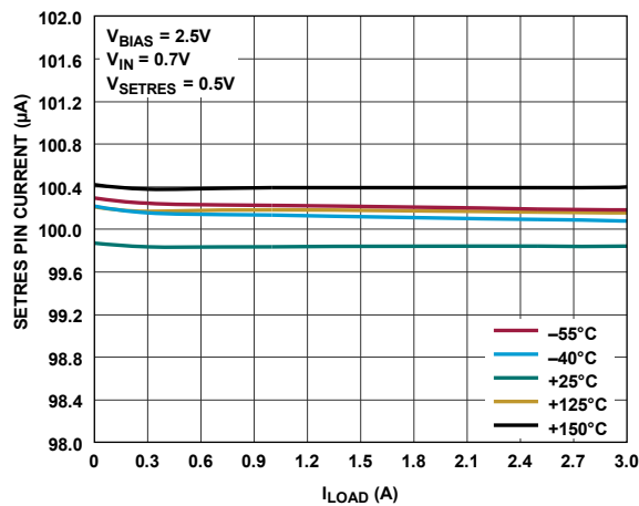
Figure 10. I_{\text{SETRES}} Load Regulation
