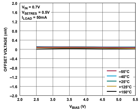
Figure 13. V_{\text{OS}} Line Regulation
