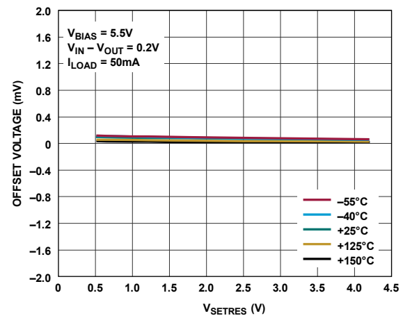
Figure 15. V_{\text{OS}} Common Mode Regulation
