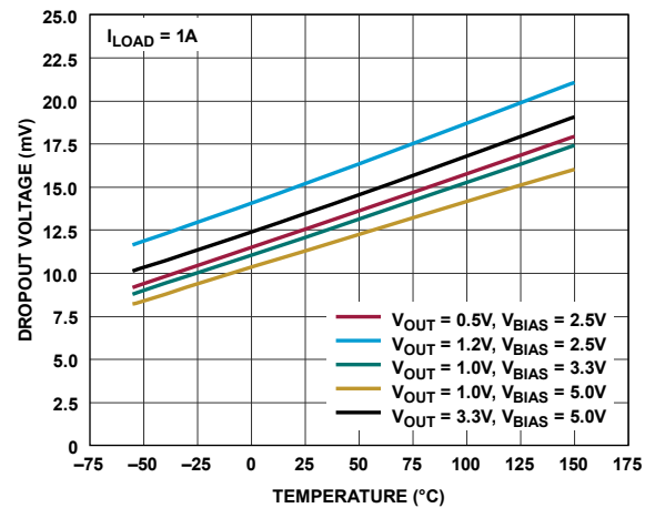
Figure 19. Dropout Voltage vs. Temperature (1A)
