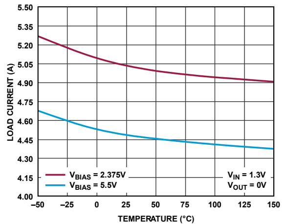
Figure 43. Internal Current Limit
