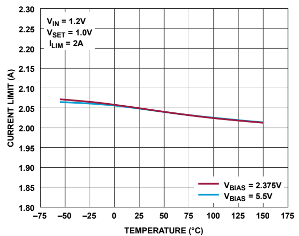
Figure 45. Programmable ILIM at 2A
