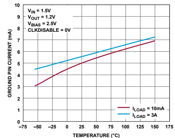
Figure 21. IGND vs. Temperature
