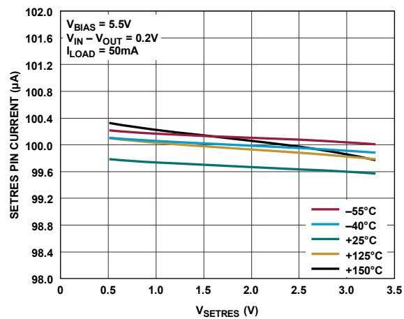
Figure 11. I_{\text{SETRES}} Common Mode Regulation
