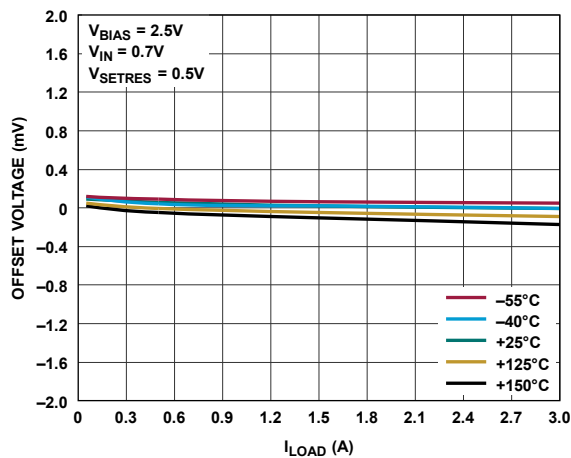
Figure 14. V_{\text{OS}} Load Regulation
