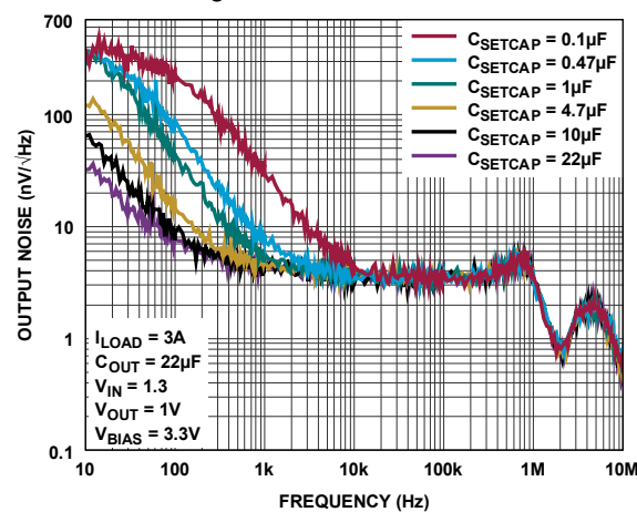
Figure 63. Noise Spectral Density
