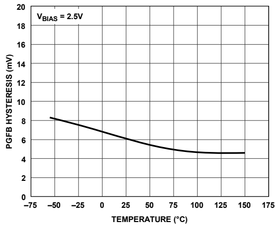
Figure 34. PGFB Hysteresis
