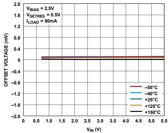
Figure 12. V_{\text{OS}} Line Regulation
