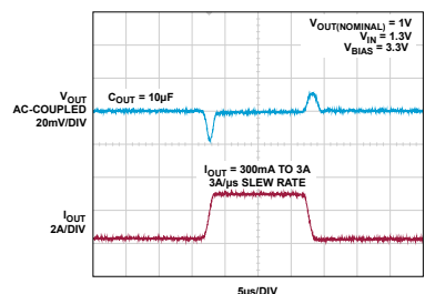
Figure 2. Transient Response
