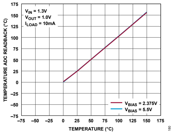
Figure 80. Temperature ADC Readback
