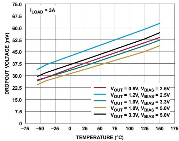
Figure 17. Dropout Voltage vs. Temperature (3A)
