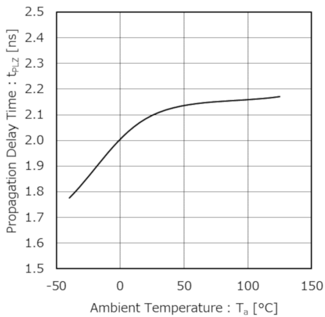
Figure 2. Propagation Delay Time: t_{PLZ} vs Ambient Temperature: T_a ( V_{CC} = 3.3\text{ V} )
