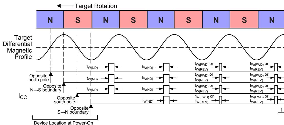
Figure 14: Calibration Behavior of the -xSxPH Variant
