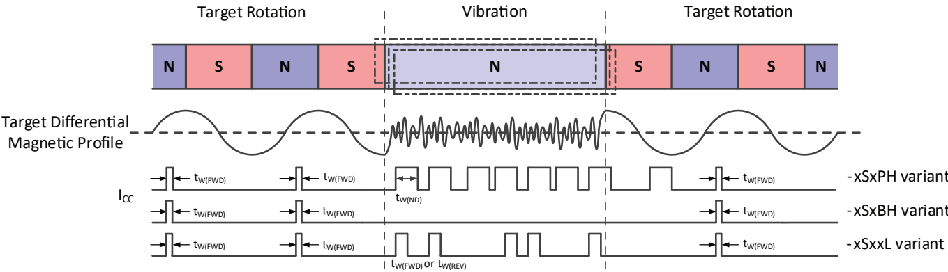
Figure 16: Vibration Behavior
