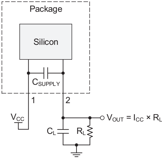
Figure 2: Application Circuit
