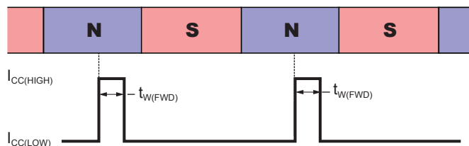
Figure 12: Output Timing Example (-xSxxx variant)
