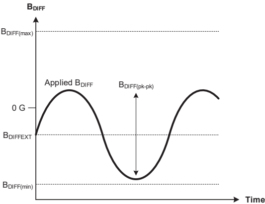
Figure 7: Input Signal Definition
