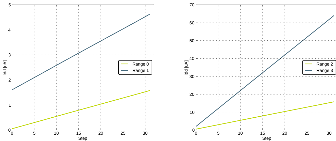
Figure 4.36. IDAC Linearity
