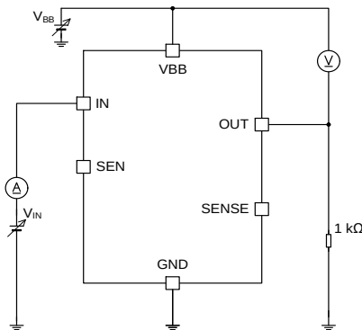
Figure 46. UVLO Threshold / Hysteresis Voltage High / Low Level Input Voltage (IN) Input Hysteresis Voltage (IN) High / Low Level Input Current (IN)
