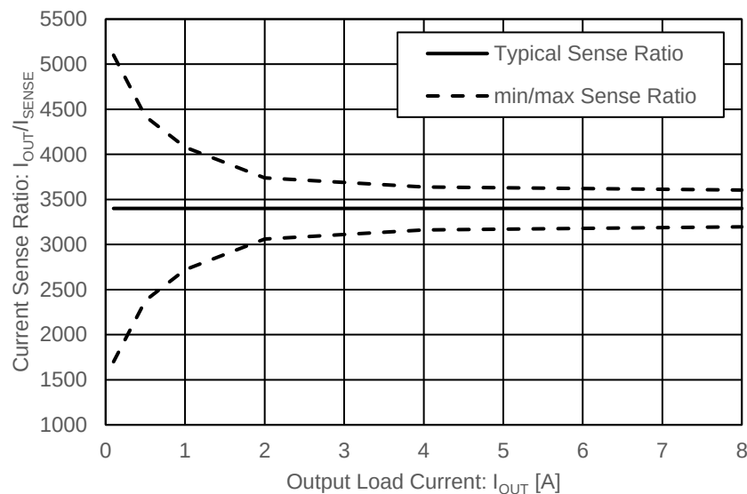
Figure 68. Current Sense Ratio vs Output Load Current
