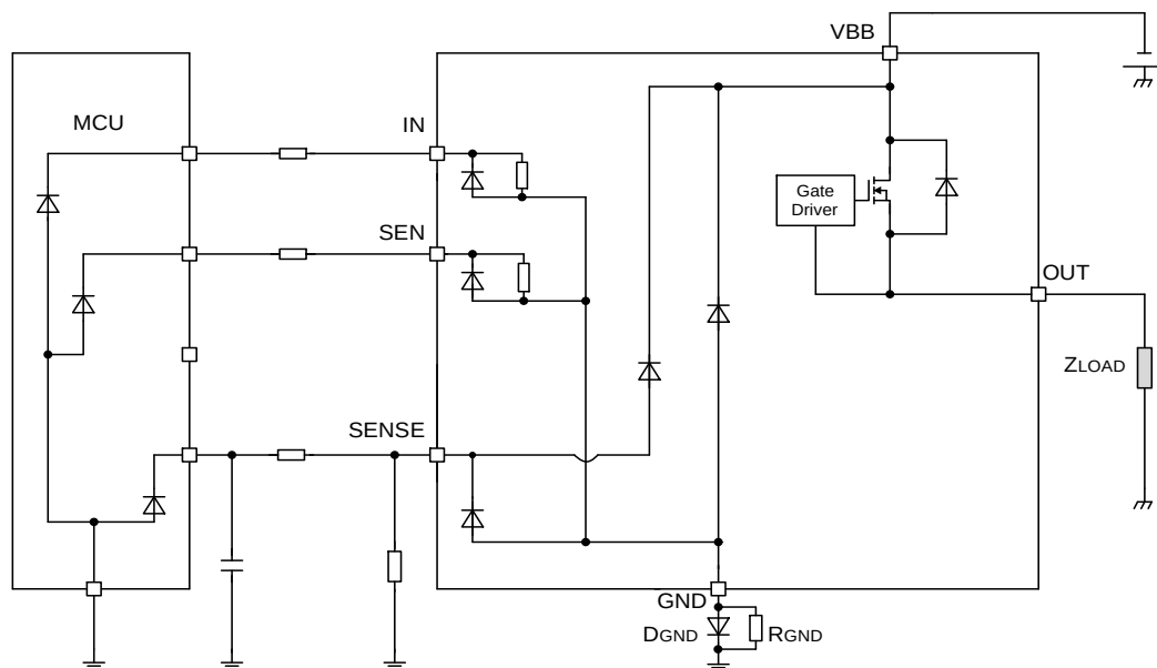
Figure 64. Reverse Battery Diagram
