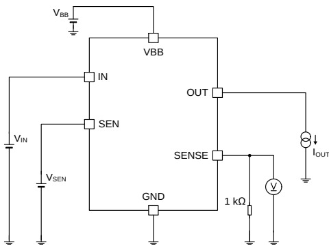
Figure 55. Current Sense Ratio
