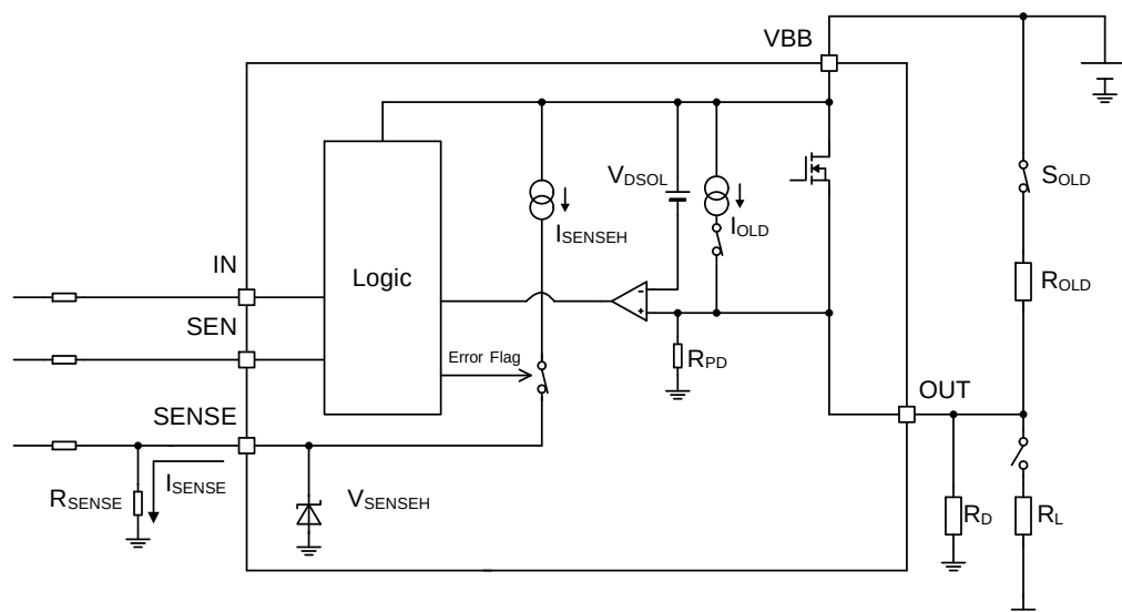
Figure 69. Open Load Detection Block Diagram
