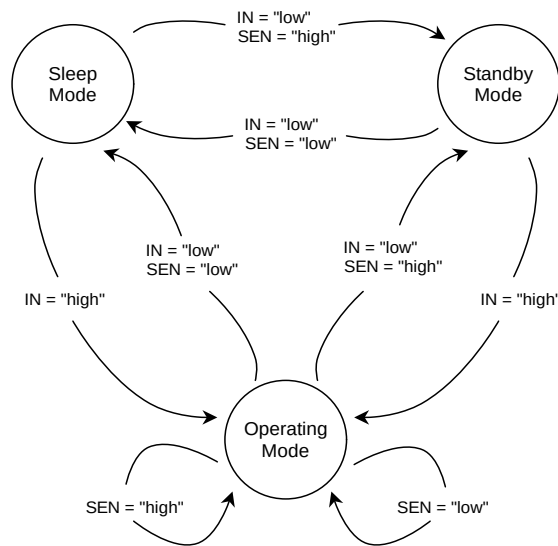
Figure 57. State Diagram
