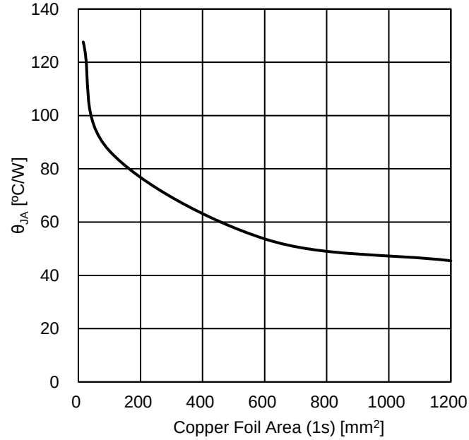
Figure 9. Thermal Resistance
