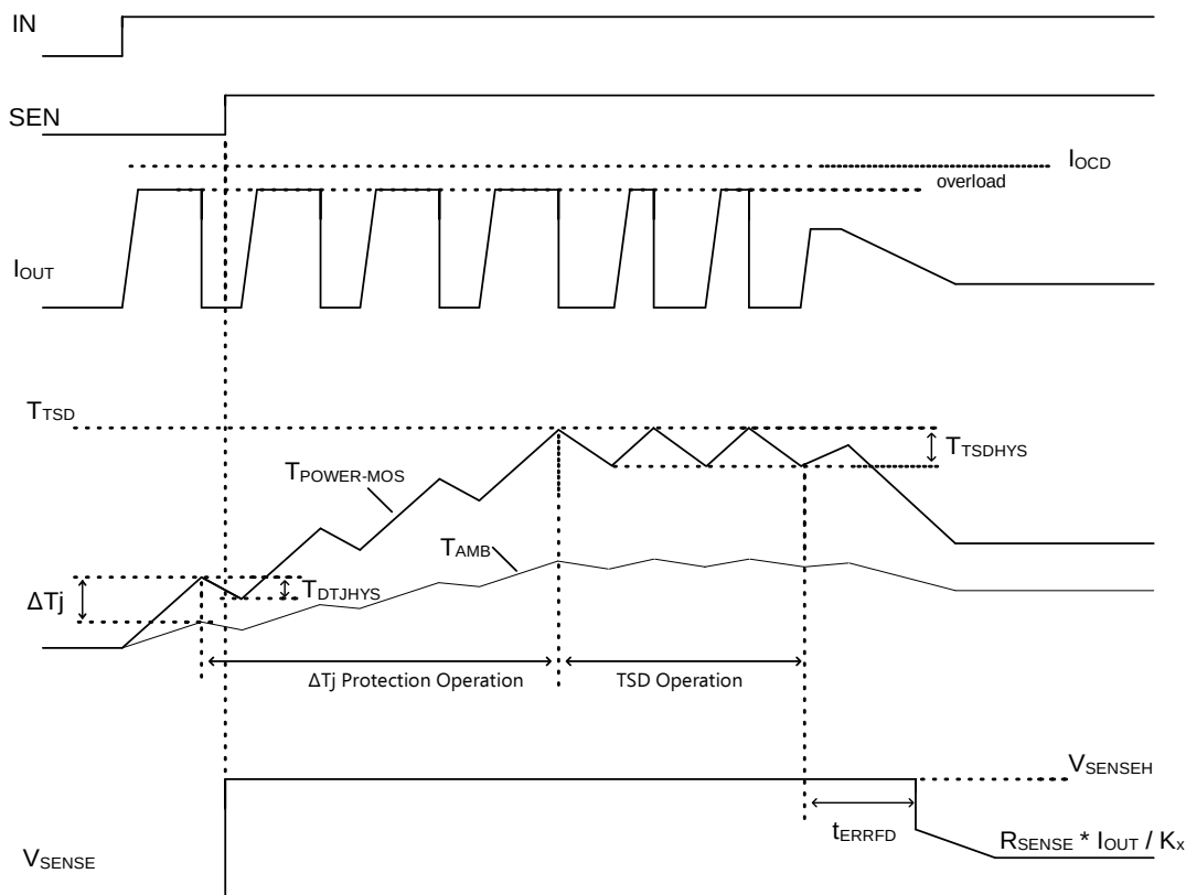
Figure 65. Overtemperature Protection
