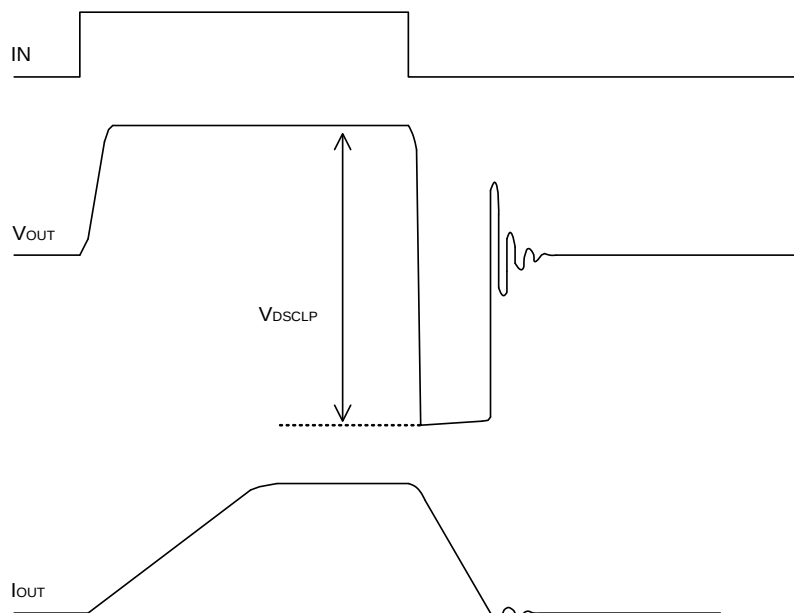
Figure 60. Switching Inductive Loads
