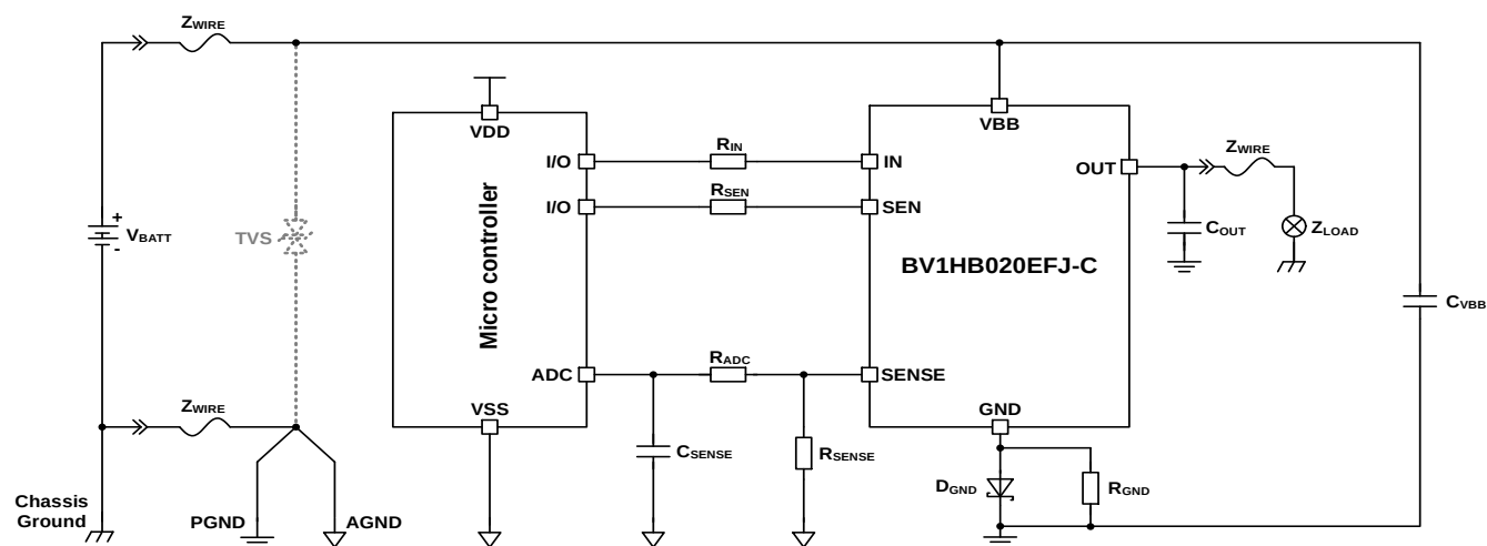
Figure 72. Application Schematic
