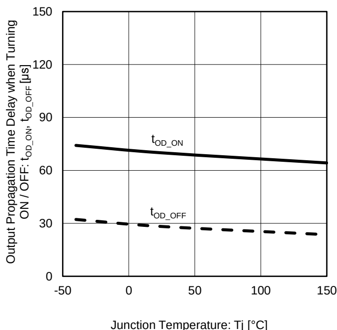
Figure 27. Output Propagation Time Delay when Turning ON / OFF vs Junction Temperature
