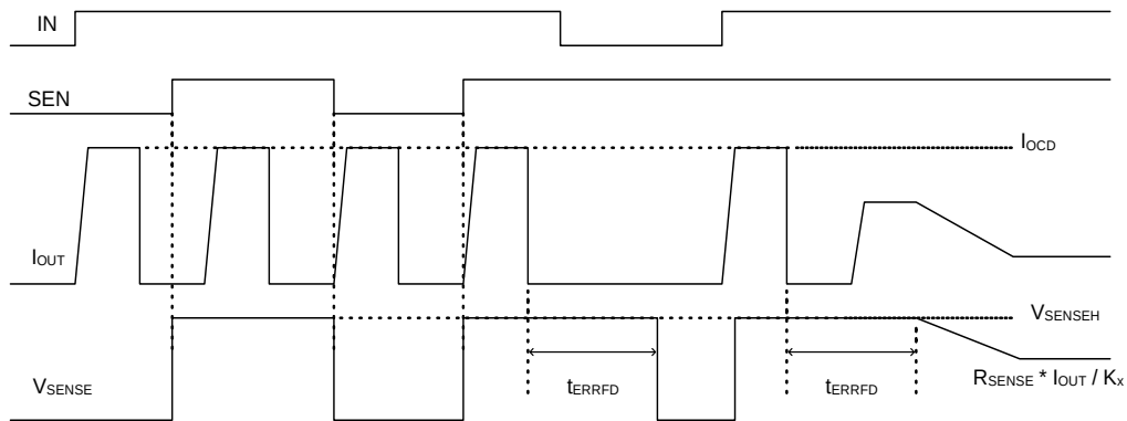
Figure 66. Overcurrent Protection
