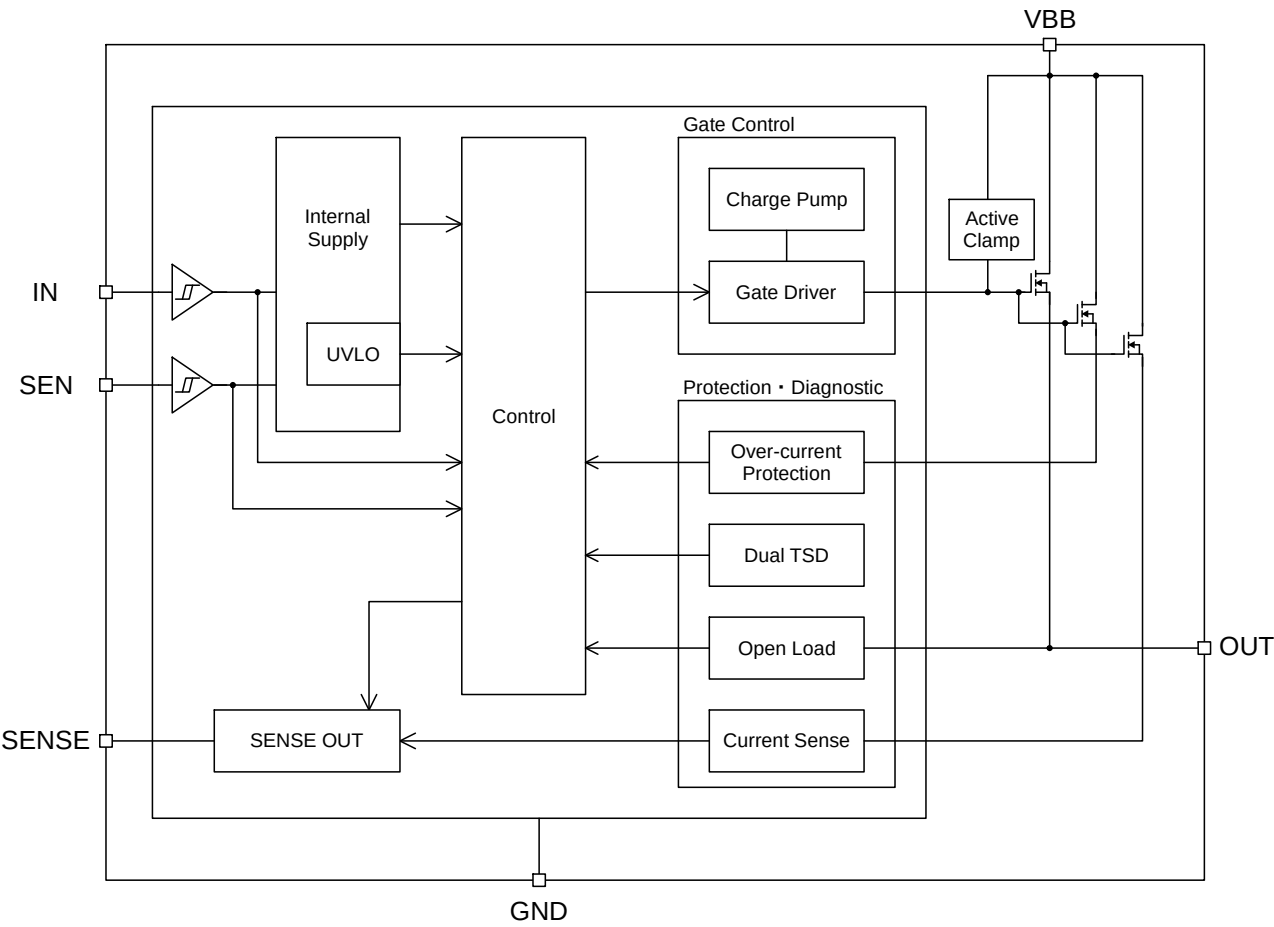
Figure 56. Block Diagram
