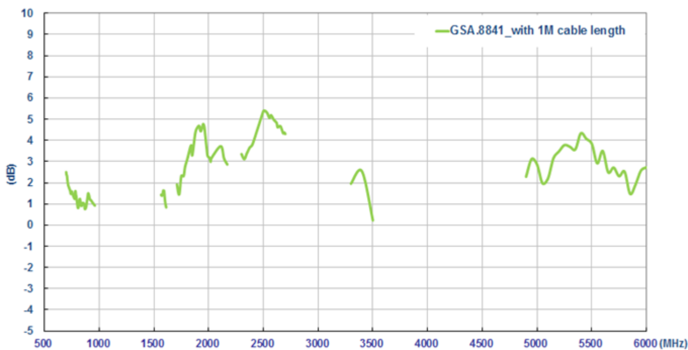
Figure9. Peak gain of GSA.8841 with 1 meter cable length on the 2mm ABS base
