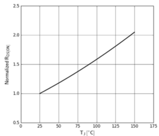
Figure 5. Normalized On-resistance
