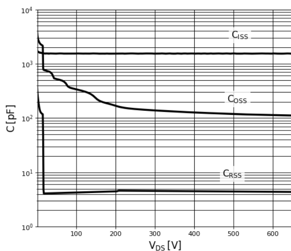
Figure 6. Typical Capacitance
