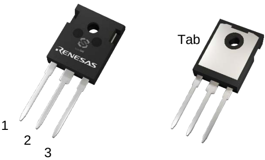
Figure 1. Pin Assignments – Bottom View
