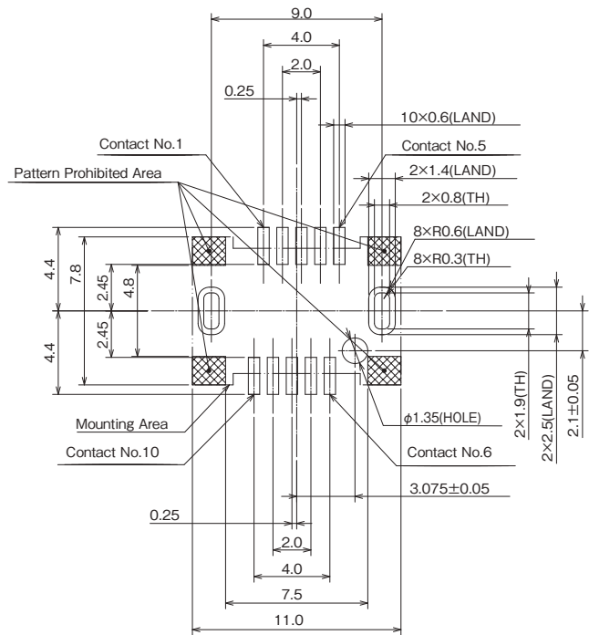
Reference Board Mounting Dimensions (From Mounting Side) (t=1.6)
