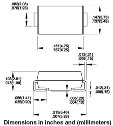
DO-214AA (SMB)
