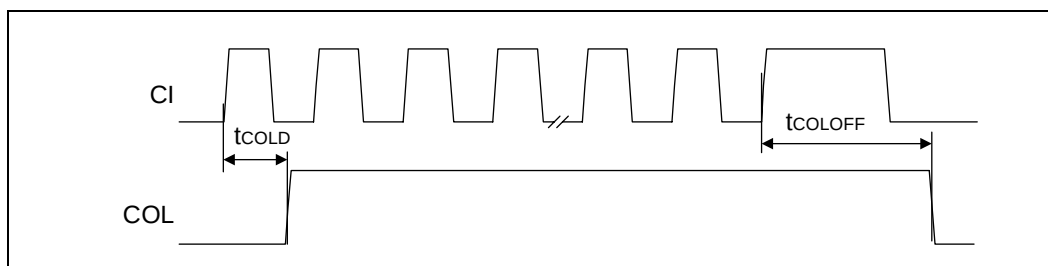
Figure 44. Mode 5 COL/SQE Output Timing
