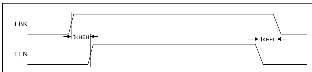
Figure 39. Mode 4 Loopback Timing
