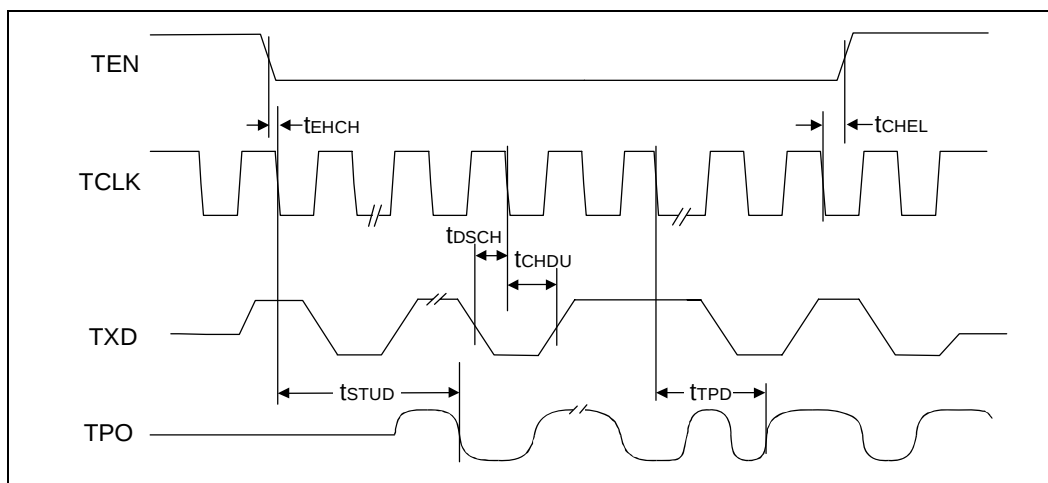
Figure 25. Mode 2 Collision Detect Timing
