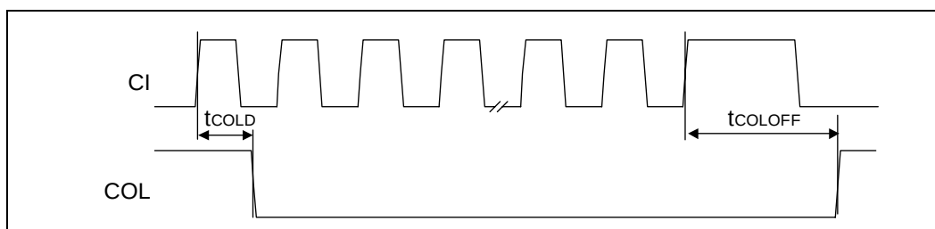
Figure 26. Mode 2 COL/SQE Output Timing
