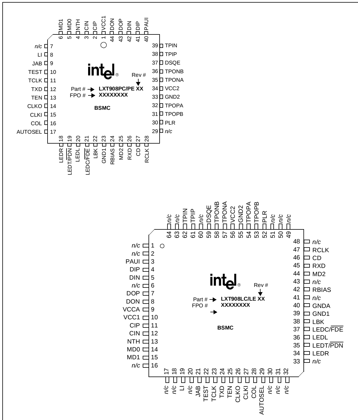
Figure 2. Pin Assignments
