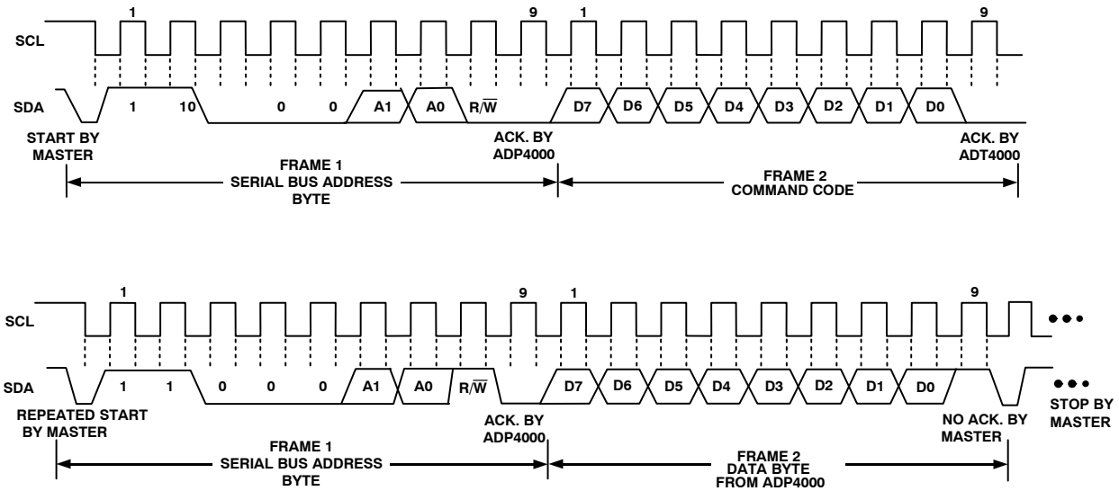
Figure 13. Read Byte
