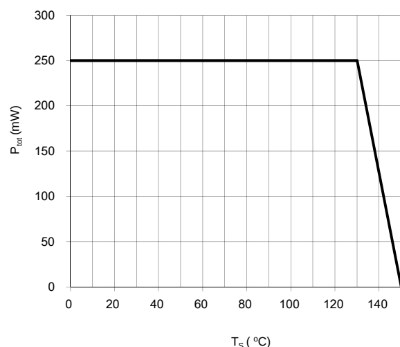
Fig.1 Total Power Dissipation P_{tot} = f(T_s)
