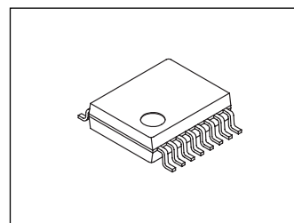
SSOP16(225mil)
