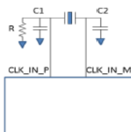
Figure 3-1 XTAL Connection
