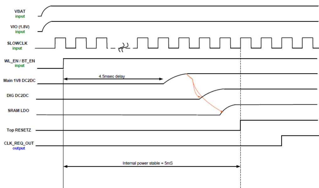
Figure 3-4 Chip Top-level Power Up Sequence
