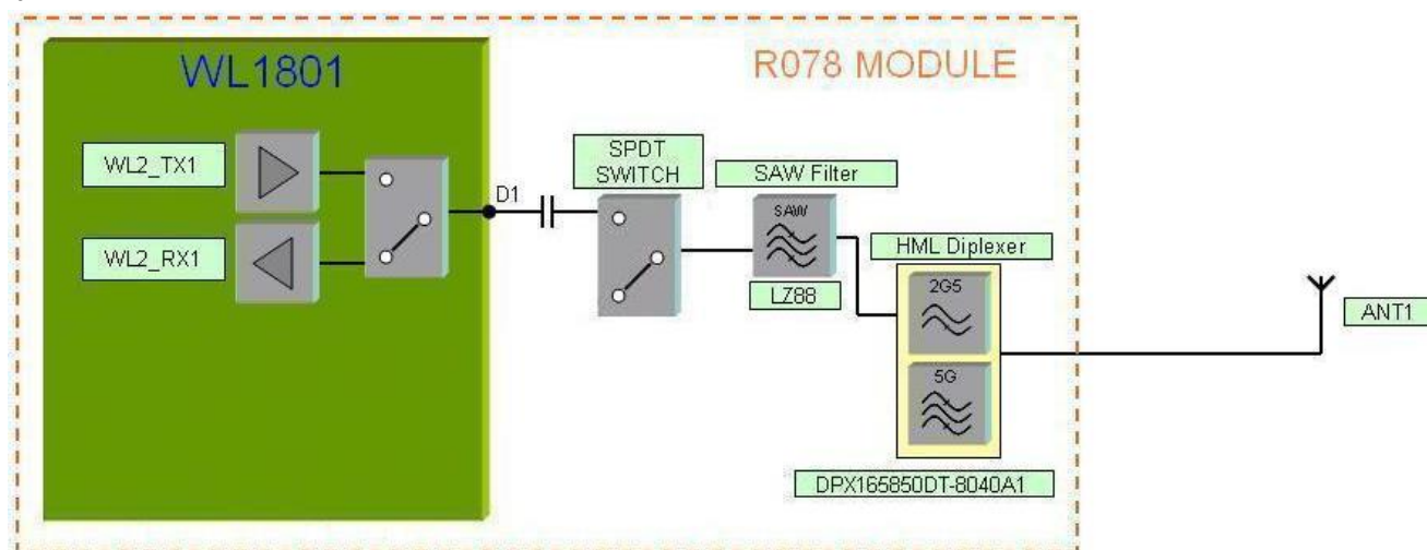
Figure 3-6 R078 (WL1801) / D7021 SISO configuration
