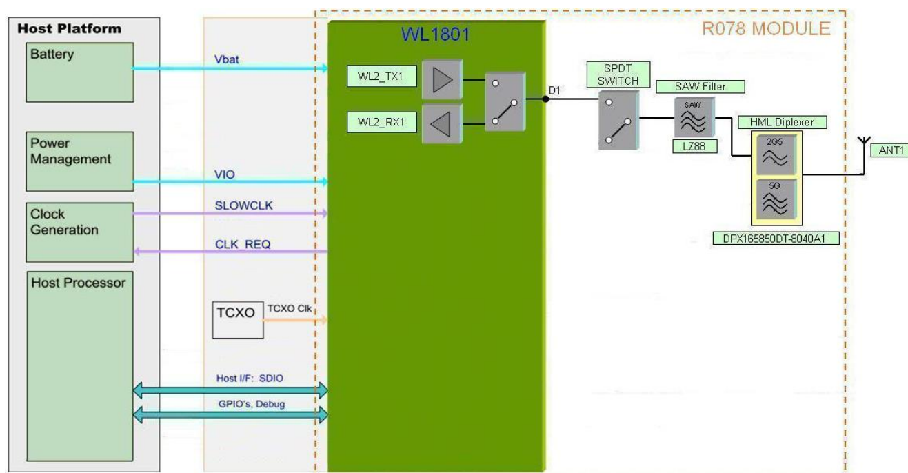
Figure 2-1 High-Level System Diagram
