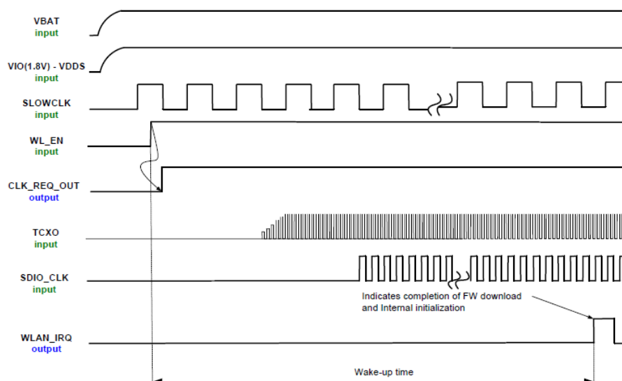
Figure 3-5 WLAN Power Up Sequence
