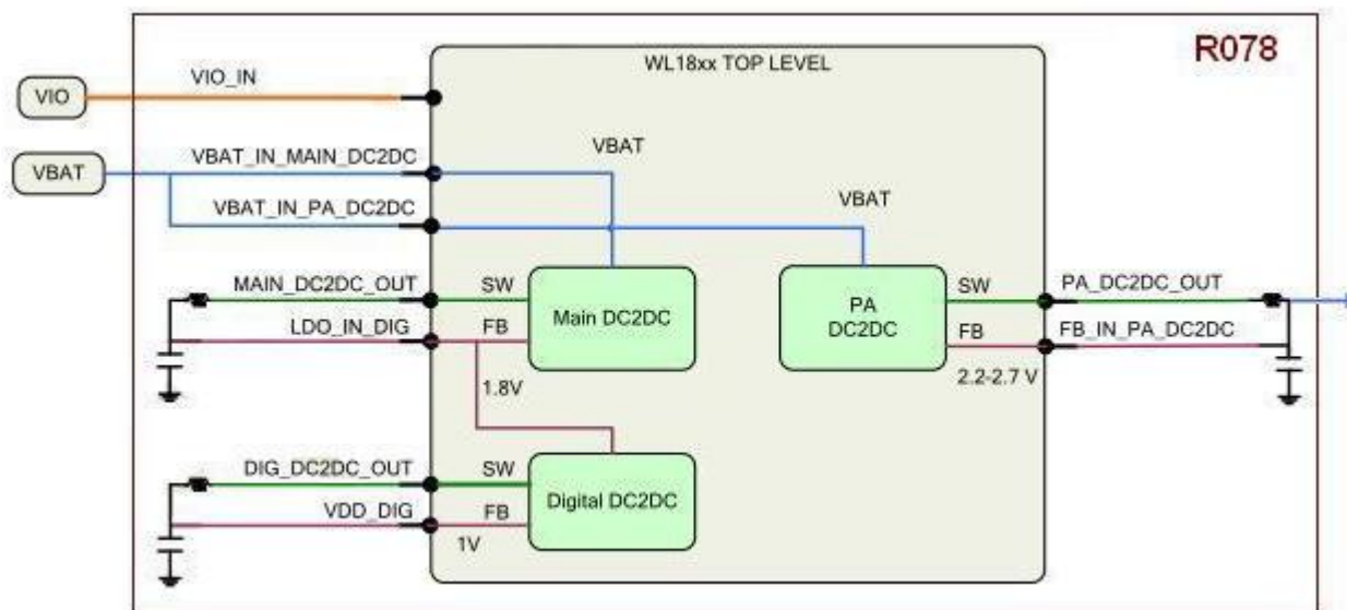
Figure 3-3 Internal DC2DC's
