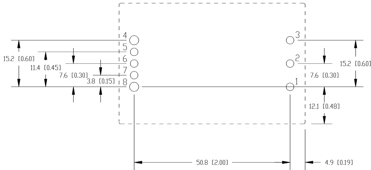
(Pin Side Down – Non-Flanged Baseplate)
