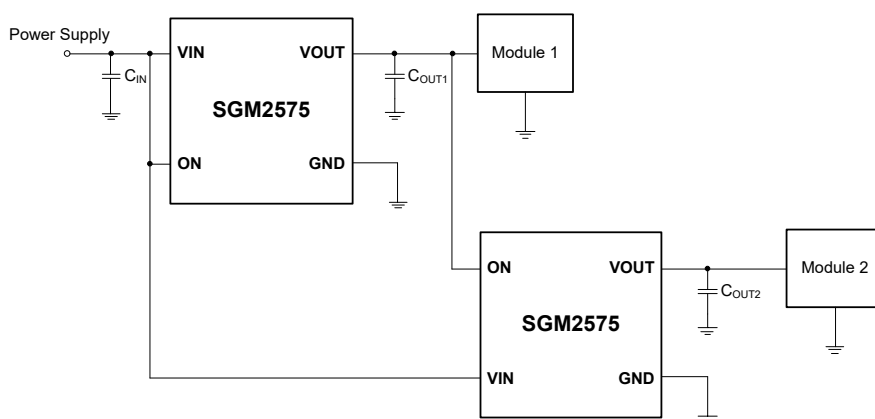
Figure 6. Power Supply Sequencing without a GPIO Input
