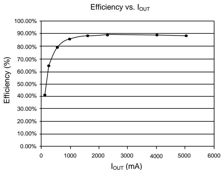
Figure 10 · Output Efficiency @ V_{OUT}=5V , V_{IN}=12V
