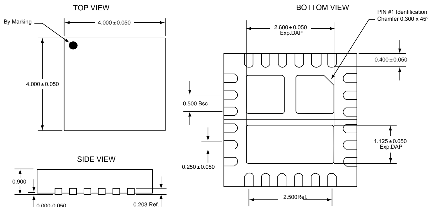
Figure 17 · Package Dimensions
