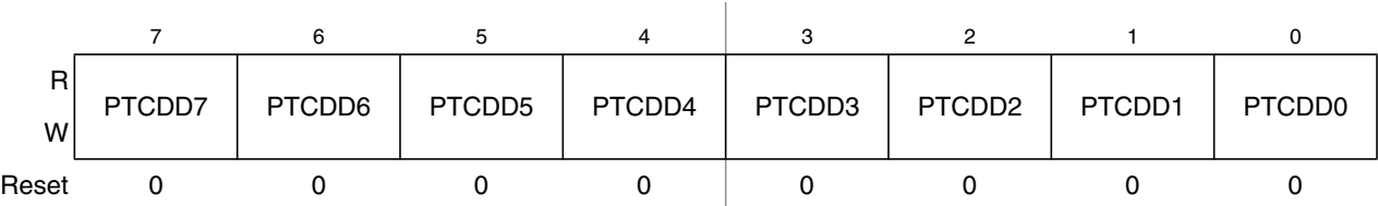
Figure 6-14. Data Direction for Port C (PTCDD)
