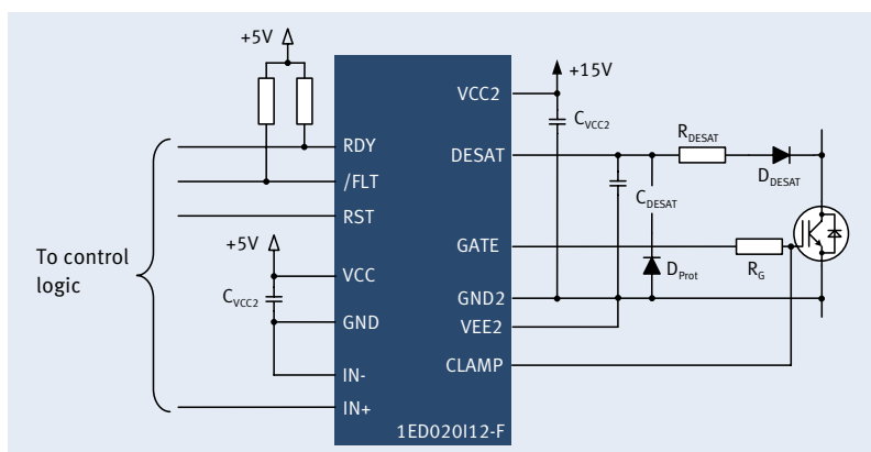
Typical application 1ED020I12-F
