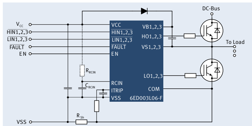
Typical application 6ED003L06-F
