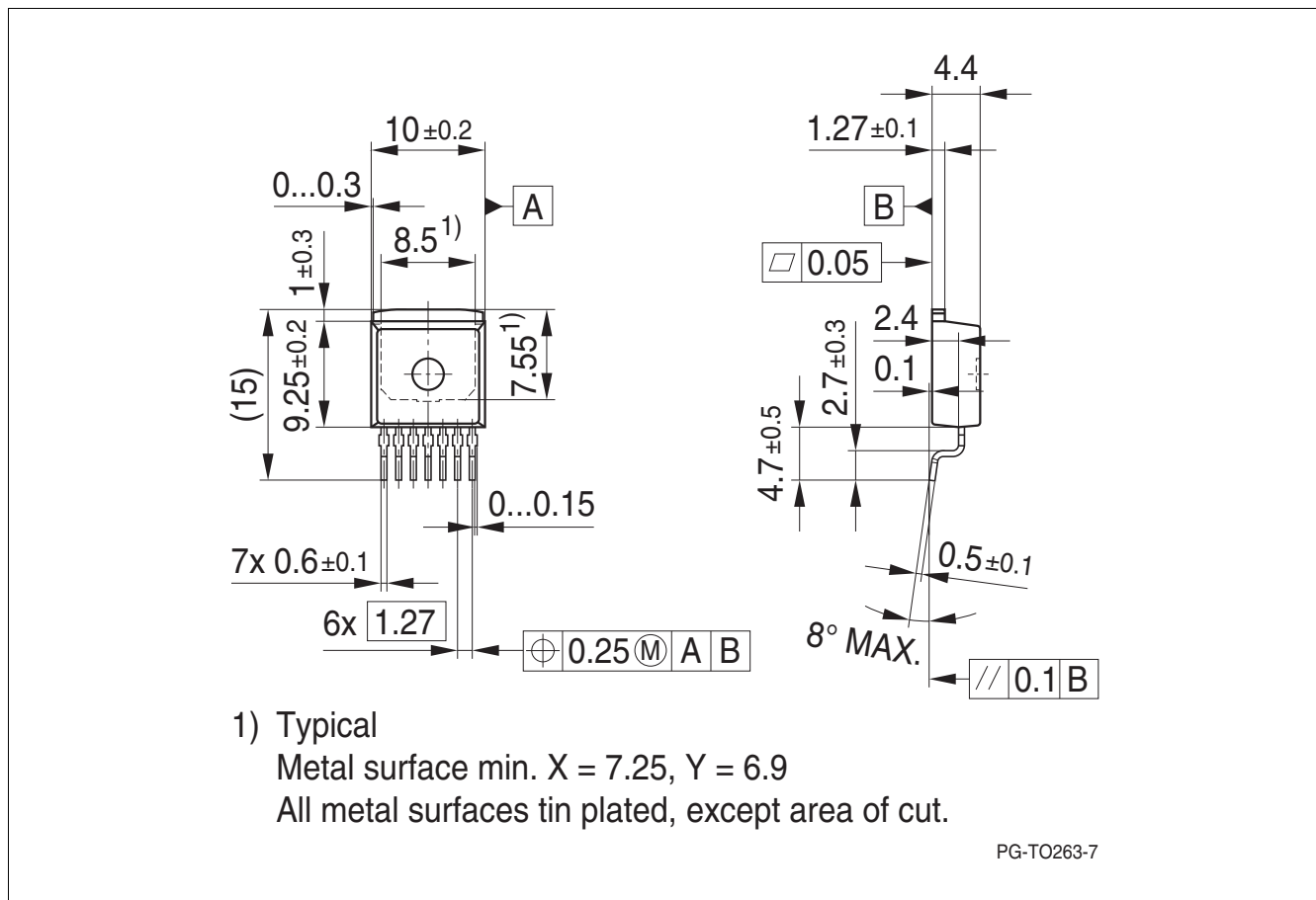
Figure 13 PG-T0263-7¹)
