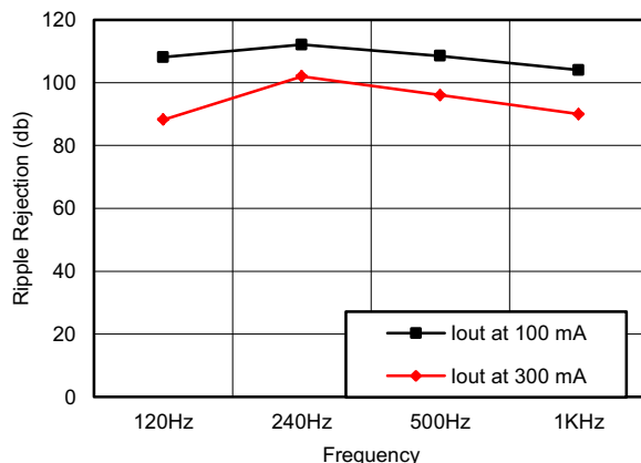
Figure 1. Ripple Rejection vs Frequency V_{\text{INPUT}} = 8\text{ V to }18\text{ V} , T_A = 25^\circ\text{C}
