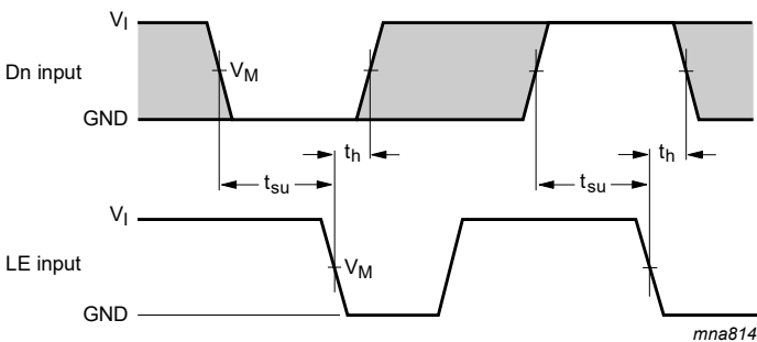
Measurement points are given in Table 8. The shaded areas indicate when the input is permitted to change for predictable output performance. V_{OL} and V_{OH} are typical output voltage levels that occur with the output load.
