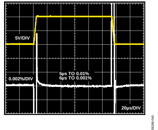
Figure 39. Large Signal Pulse Response and Settle Time, G = 1 , R_{LOAD} = 10\text{ k}\Omega , V_S = \pm 15\text{ V} , V_{REF} = 0\text{ V}
