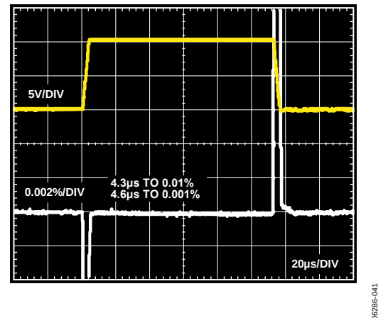
Figure 40. Large Signal Pulse Response and Settle Time, G = 10 , R_{LOAD} = 10\text{ k}\Omega , V_S = \pm 15\text{ V} , V_{REF} = 0\text{ V}
