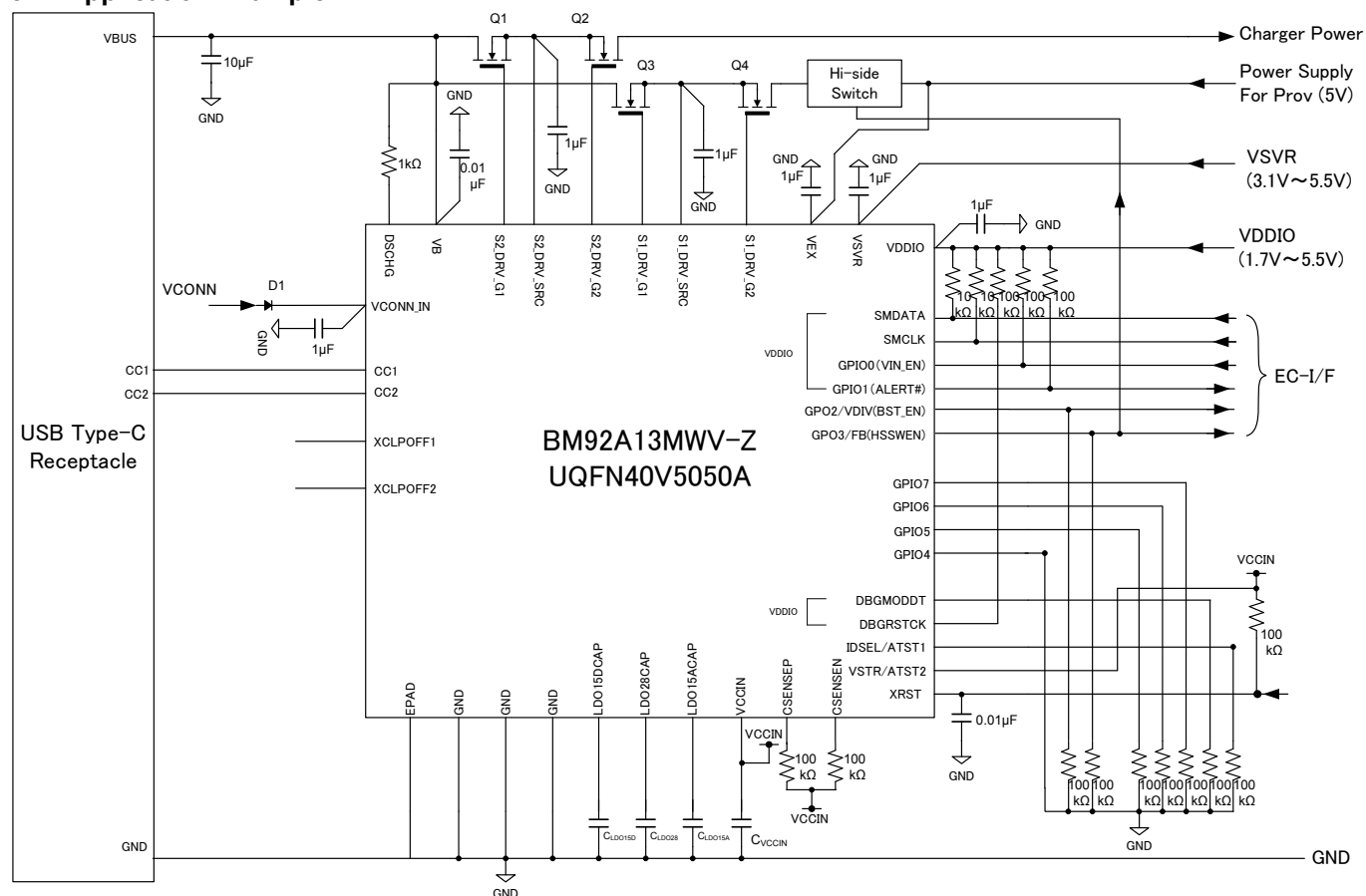
Figure 5-1 Application Example
