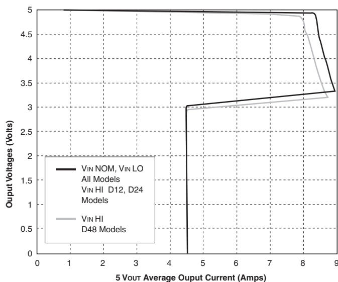
Figure 2b. Current Limiting Characteristics for 5V Output
