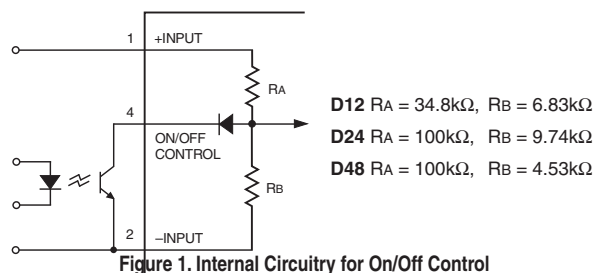
Figure 1. Internal Circuitry for On/Off Control
