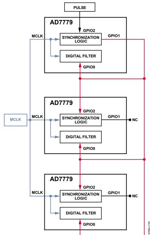
Figure 110. Hardware ODR
