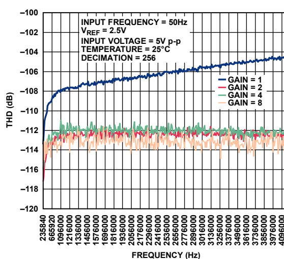
Figure 37. THD vs. MCLK Frequency, Low Power Mode, Input Frequency ( f_{IN} ) = 50 Hz, Decimation = 256
