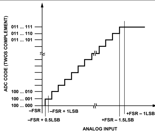
Figure 91. Transfer Function
