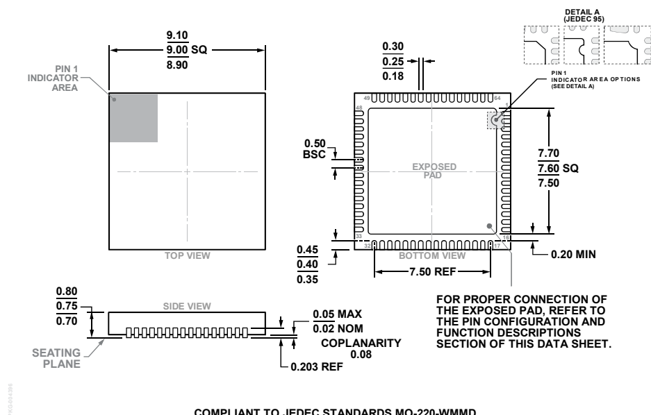
COMPLIANT TO JEDEC STANDARDS MO-220-WMMD Figure 124. 64-Lead Lead Frame Chip Scale Package [LFCSP] 9 mm × 9 mm Body and 0.75 mm Package Height (CP-64-15) Dimensions shown in millimeters
