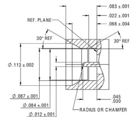
SMPM (Full Detent) Male PER MIL-STD-348A - Figure 328.2
