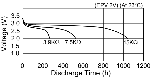
Figure 1. Discharge Characteristics
