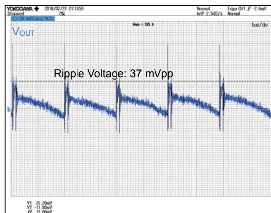
Figure 22. V_{IN} = 230 \text{ Vac} , I_{OUT} = 0.15 \text{ A}
