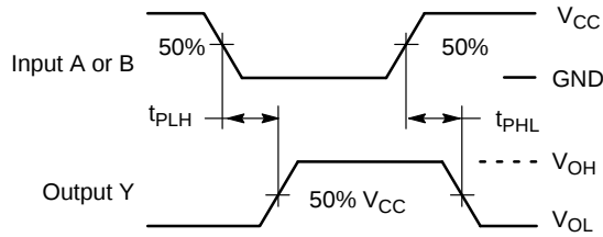
Figure 3. Switching Waveforms
