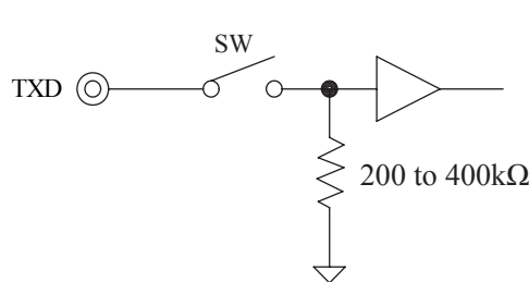
* TXD Equipment circuit
