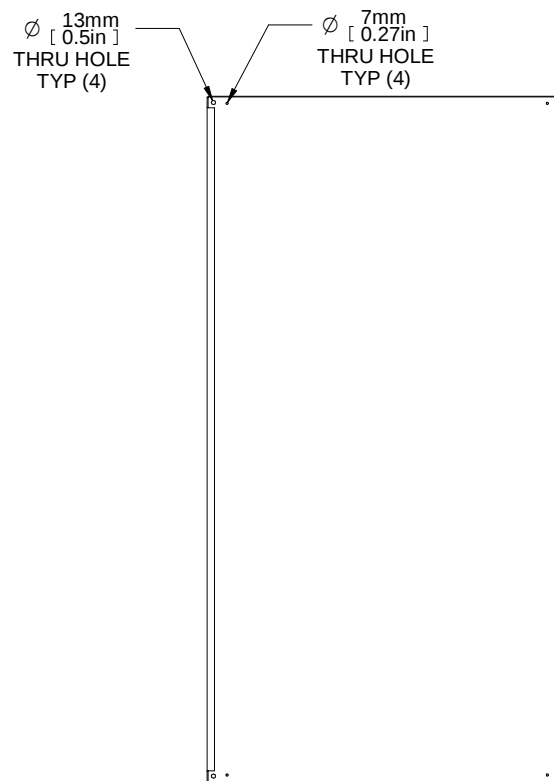
REAR VIEW
