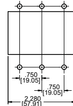
MountingDetail*
