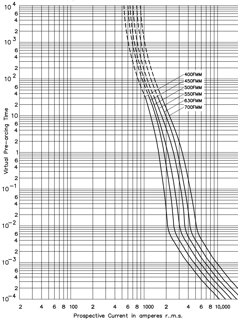
Time-current curve - FMM, 400 A to 700 A
