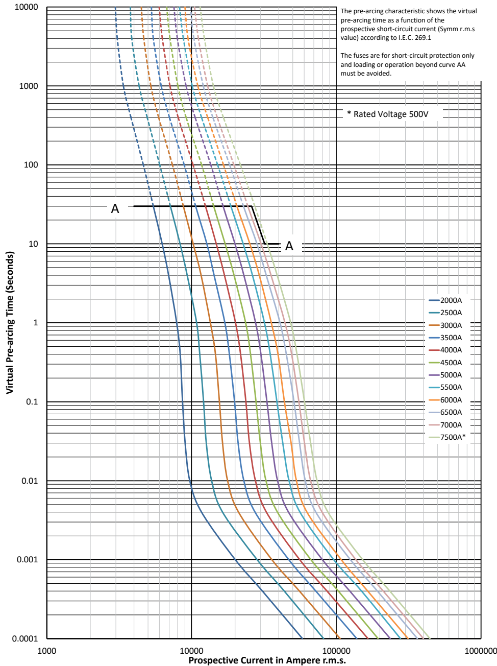
Time-current curve - 2000 A to 7500 A
