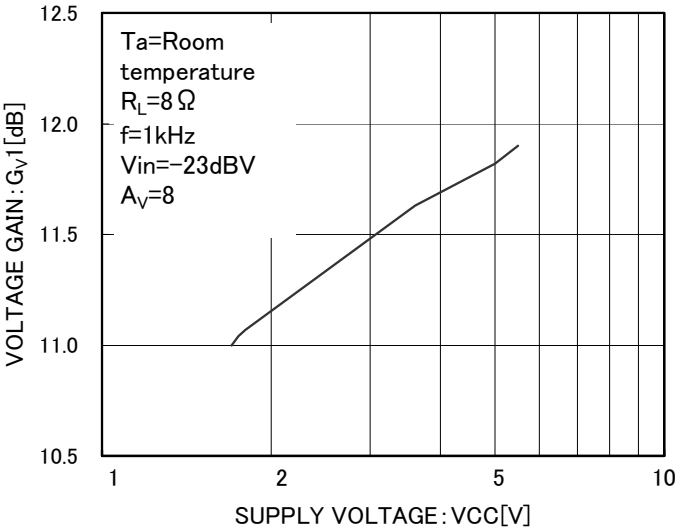
Fig.26 Gain(1stAmp) — Power supply
