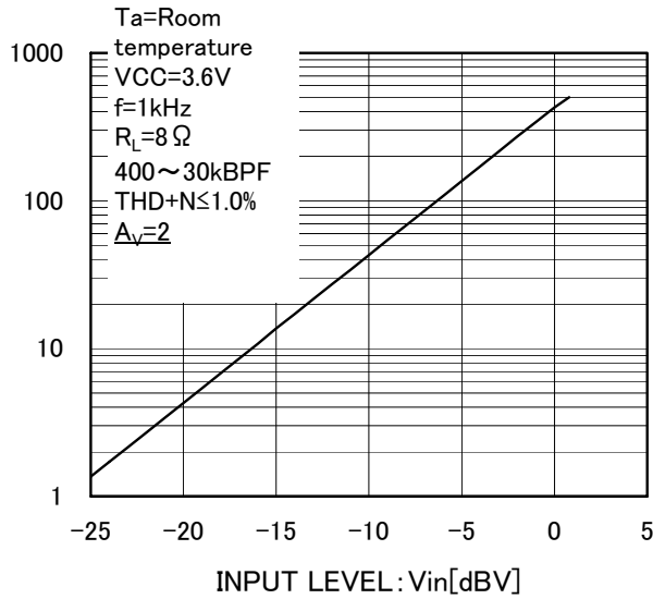
Fig.17 Output Power — Input level
