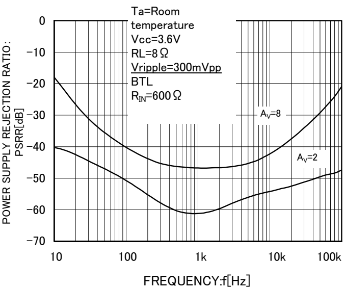
Fig.31 Power Supply Rejection Ratio — Frequency
