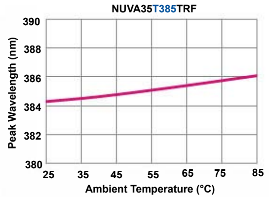
AMBIENT TEMPERATURE VS. PEAK WAVELENGTH @ 500mA If
