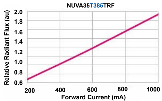
FORWARD CURRENT VS. RELATIVE RADIANT FLUX @ +25°C
