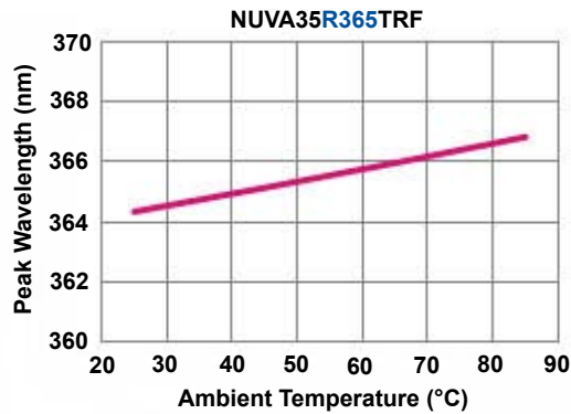
AMBIENT TEMPERATURE VS. PEAK WAVELENGTH @ 500mA If
