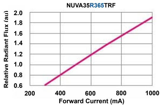
FORWARD CURRENT VS. RELATIVE RADIANT FLUX @ +25°C
