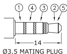
Ø3.5 MATING PLUG
