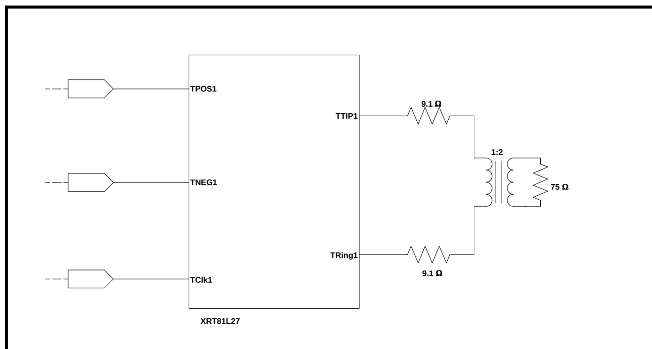
FIGURE 8. ILLUSTRATION OF HOW TO INTERFACE THE TRANSMIT SECTIONS OF THE XRT81L27 TO THE LINE (FOR 75Ω APPLICATIONS)
