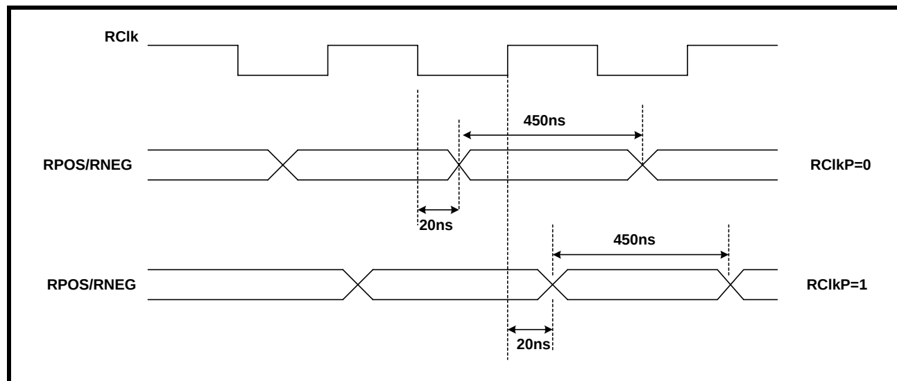
FIGURE 4. RECEIVE OUTPUT TIMING
