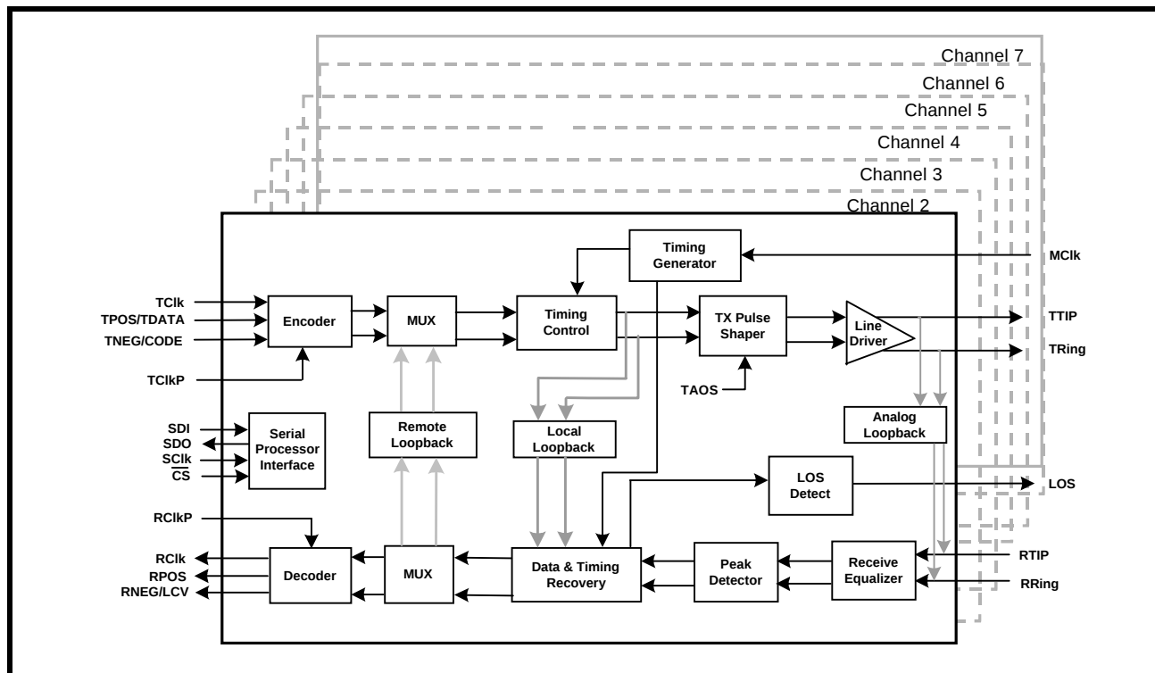
FIGURE 1. BLOCK DIAGRAM
