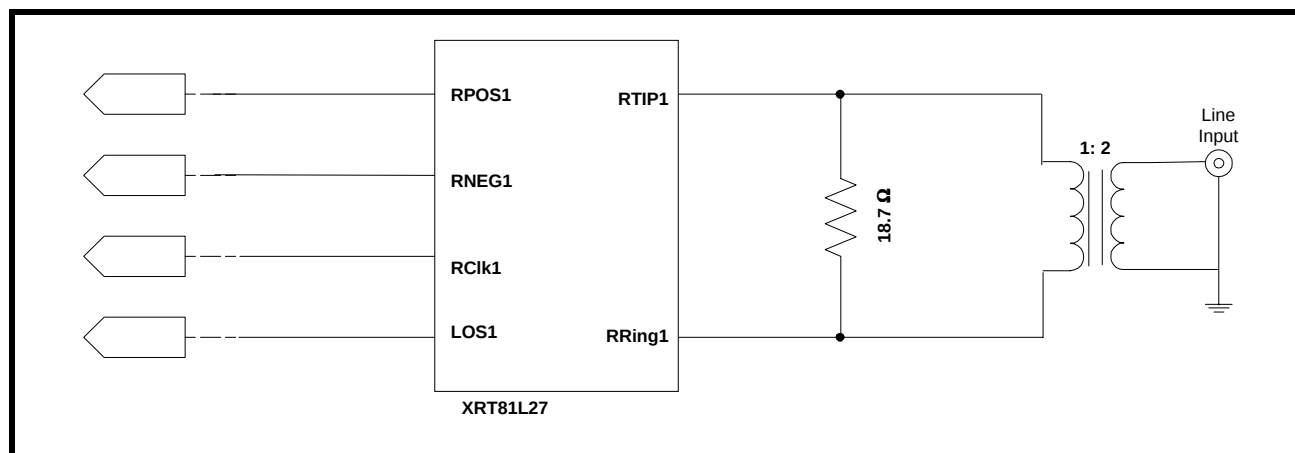
FIGURE 10. RECOMMENDED SCHEMATIC FOR INTERFACING THE RECEIVE SECTIONS OF THE XRT81L27 TO THE LINE FOR 75\Omega APPLICATIONS (TRANSFORMER-COUPLING)
