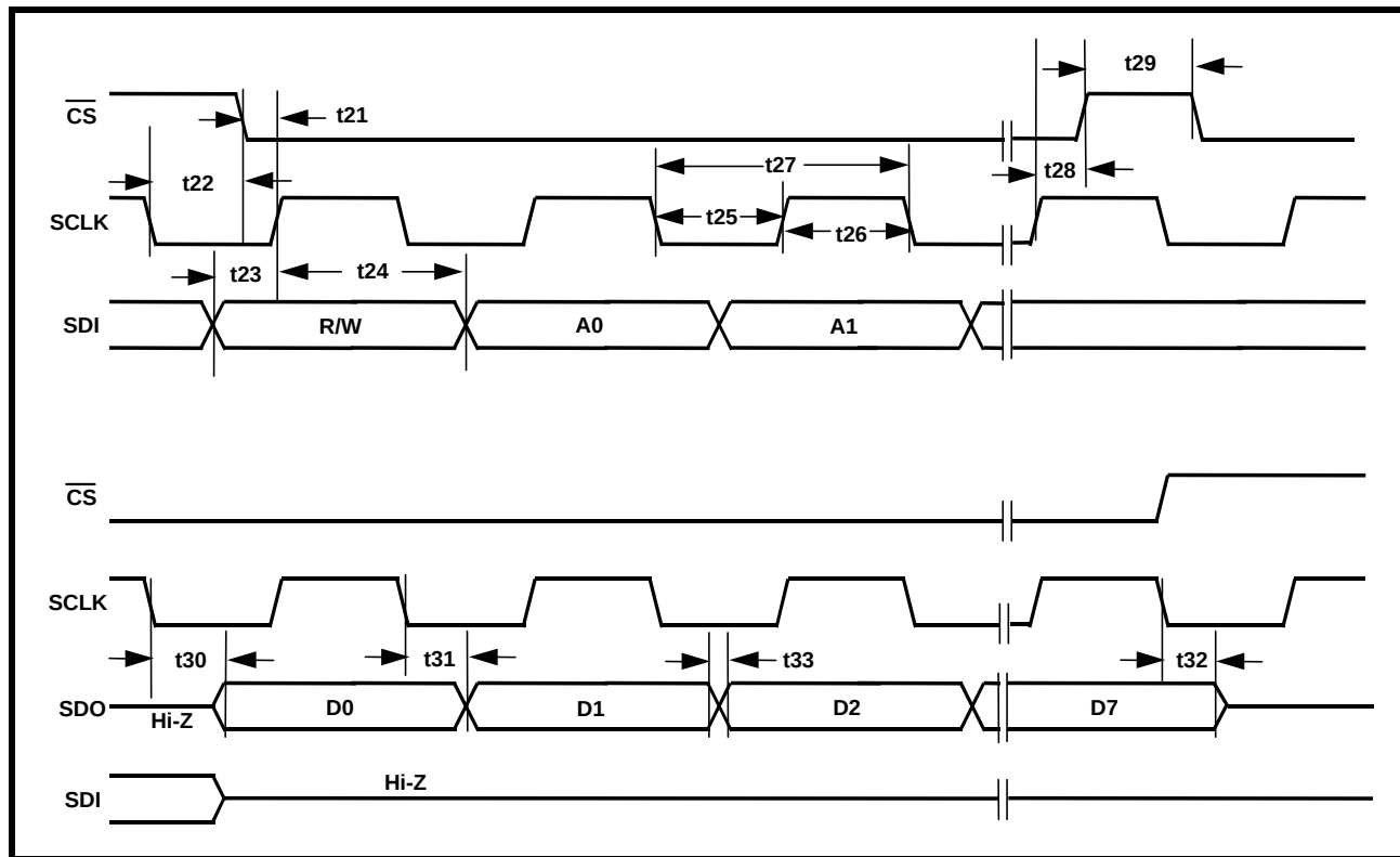
FIGURE 5. TIMING DIAGRAM FOR THE MICROPROCESSOR SERIAL INTERFACE
