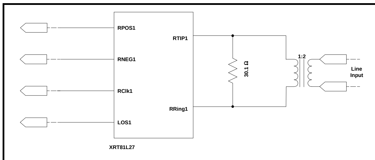
FIGURE 11. RECOMMENDED SCHEMATIC FOR INTERFACING THE RECEIVE SECTIONS OF THE XRT81L27 TO THE LINE FOR 120\Omega APPLICATIONS (TRANSFORMER-COUPLING)
