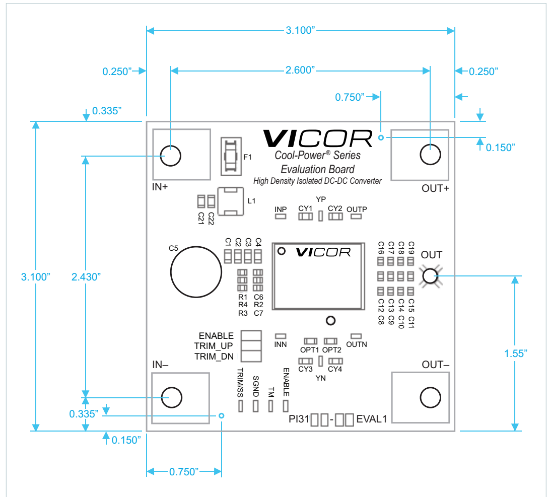
Figure 13 Mechanical drawing
