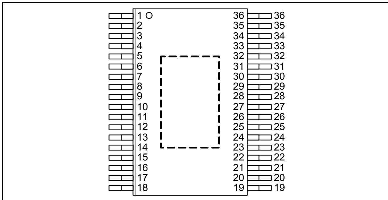
Figure 3 Pin Configuration
