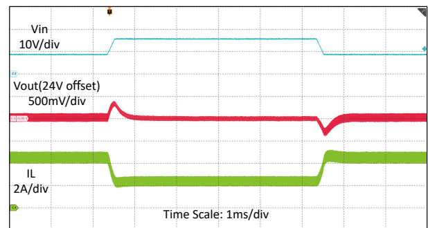
V_{OUT} = 24\text{ V} I_{OUT} = 1.5\text{ A} Figure 8-9. Line Transient ( V_{IN} = 9\text{ V} to 16\text{ V} )
