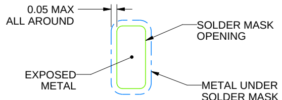
SOLDER MASK DEFINED
