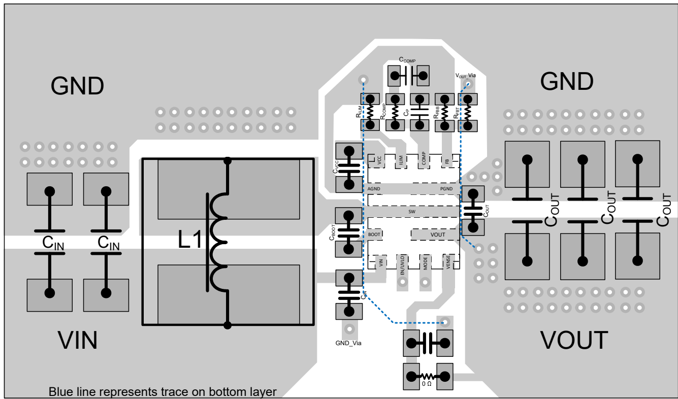
Figure 8-12. Layout Example
