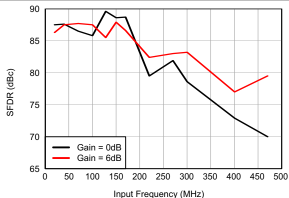
Figure 6-11. SFDR vs Input Frequency
