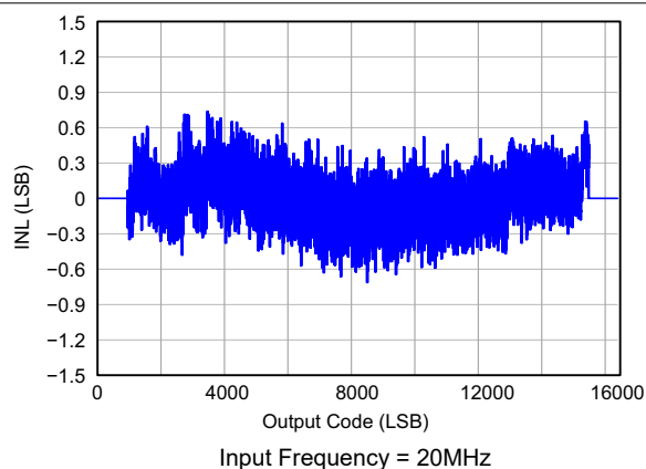
Figure 6-26. Integrated Nonlinearity
