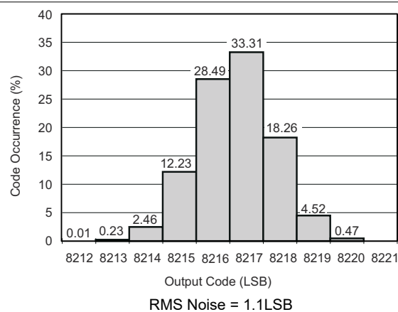
Figure 6-27. Output Noise Histogram (With Inputs Shorted To VCM)
