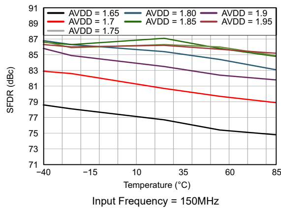
Figure 6-20. SFDR vs Temperature And AVDD Supply
