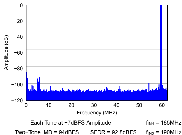
Figure 6-9. FFT For Two-Tone Input Signal
