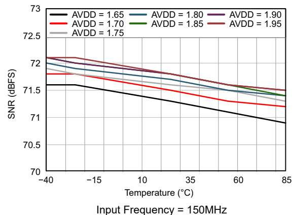
Figure 6-21. SNR vs Temperature And AVDD Supply
