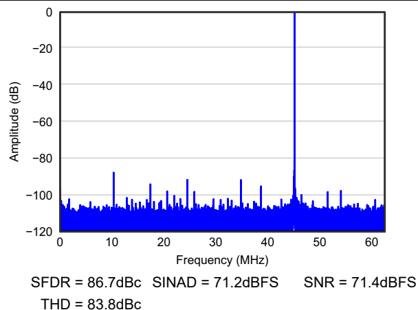
Figure 6-7. FFT For 170MHz Input Signal
