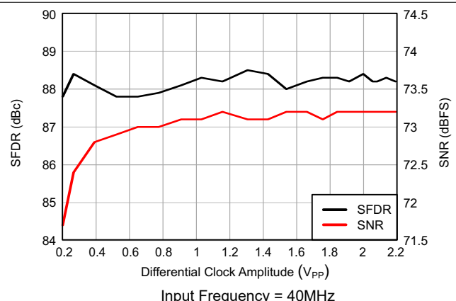
Figure 6-23. Performance vs Input Clock Amplitude
