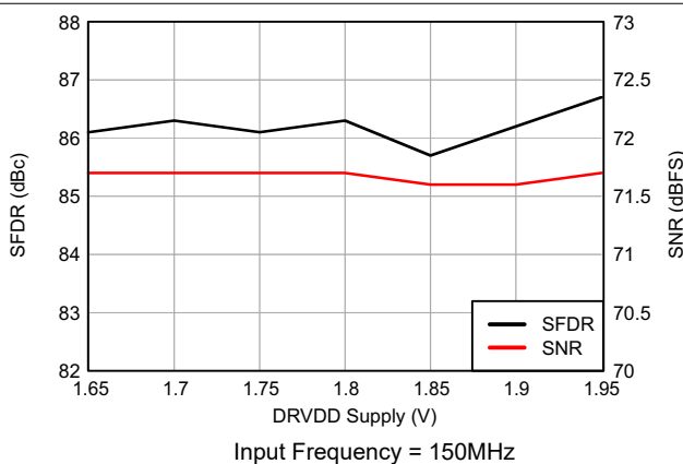
Figure 6-22. Performance vs DRVDD Supply Voltage
