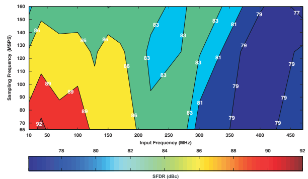
Figure 6-34. Spurious-Free Dynamic Range (6dB Gain)
