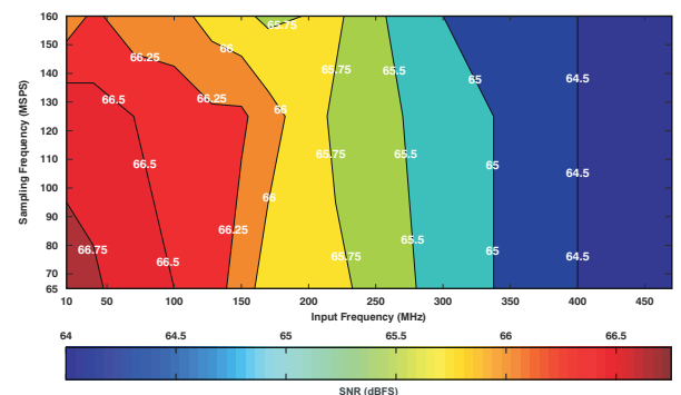
Figure 6-38. Signal-To-Noise Ratio (6dB Gain)
