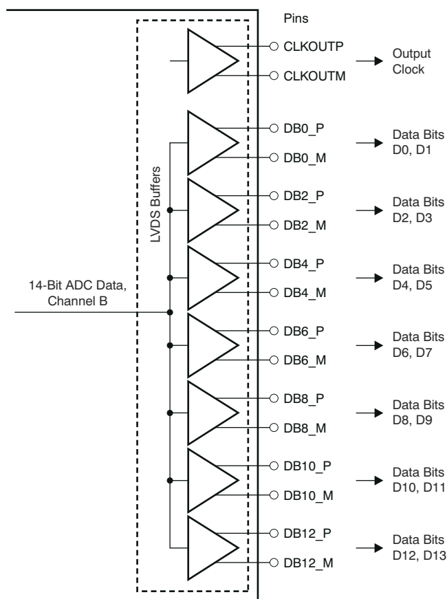
Figure 7-2. LVDS Interface
