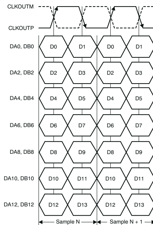
Figure 6-5. ADS4245 LVDS Interface Timing Diagram
