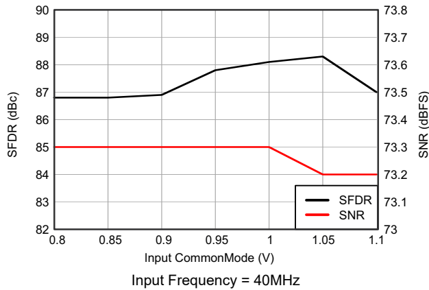
Figure 6-18. Performance vs Input Common-Mode Voltage
