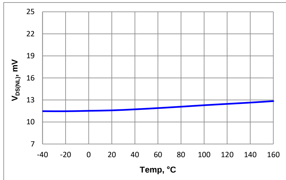
Figure 4. Output Voltage Drop Regulation, I_{OUT} = 50mA
