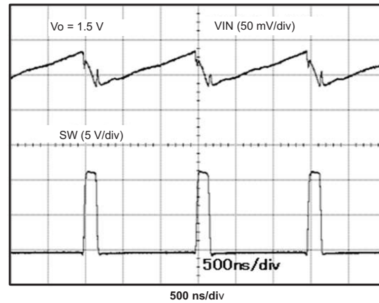
Figure 15. Voltage Ripple vs Ripple at Input ( I_O = 4 A)
